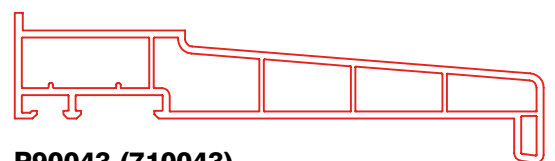
P90043 (710043) 180mm Cill
